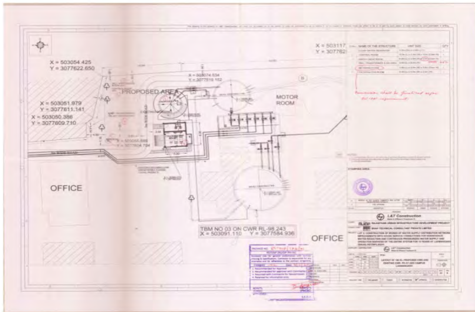
Figure 2: Layout of proposed Clear Water Reservoir at A.En. Headworks, PHED Campus
